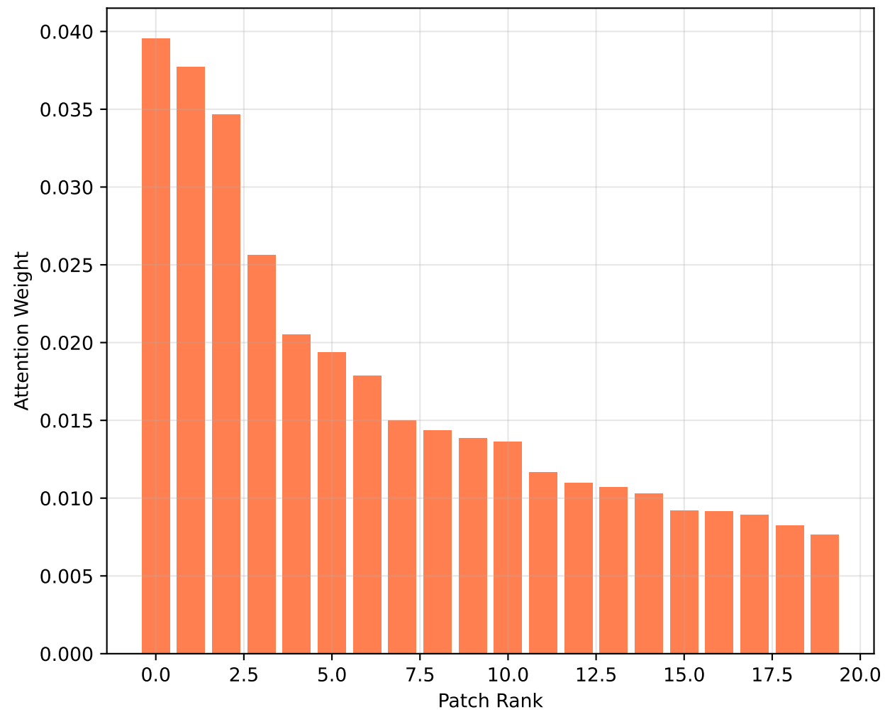
Top-20 Patches Cumulative: 0.339
